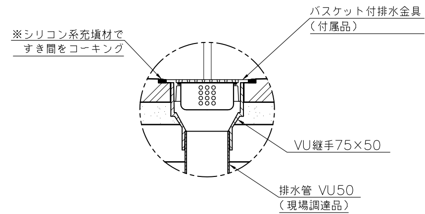
B部詳細図 (SCALE:1/5)
